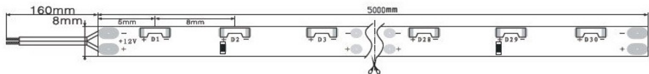
dimension diagram (unit:mm)
